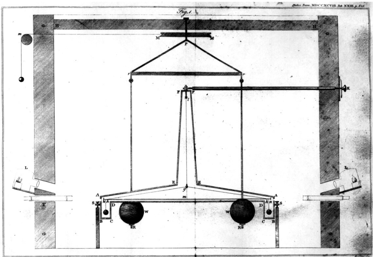
Figure 4. Cavendish's apparatus for measuring the mean density of the earth, taken from Cavendish (1798). The figure shows a vertical section 'through the instrument and the building in which it is placed. ABCDDCBAEFFE , is the case; x and x are the two balls, which are suspended by the wires xh from the arm ghmh , which is itself suspended by the slender wire gl . This arm consists of a slender deal rod hnh , strengthened by a silver wire ghg ; by which means it is made strong enough to support the balls, though very light. The case is supported, and set horizontal, by four screws, resting on posts fixed firmly into the ground: two of them are represented in the figure, by S and S ... GG and GG are the end walls of the building. W and W are the leaden weights; which are suspended by the copper rods RrPrR , and the wooded bar rr , from the centre pin Pp . This pin passes through a hole in the beam HH , perpendicularly over the centre of the instrument, and turns round in it, being prevented from falling by the plate p . MM is a pulley, fastened to this pin; and Mm , a cord wound round the pulley, and passing through the end wall; by which the observer may turn it round, and thereby move the weights from one situation to the other'. (Cavendish 1798, pp 250–1). The beam was about 6' long, the suspension wire was about 40' long and the room about 10' square.
